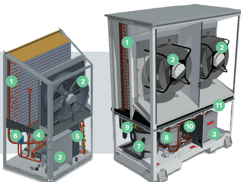
Compress 5000 AW 22 O
